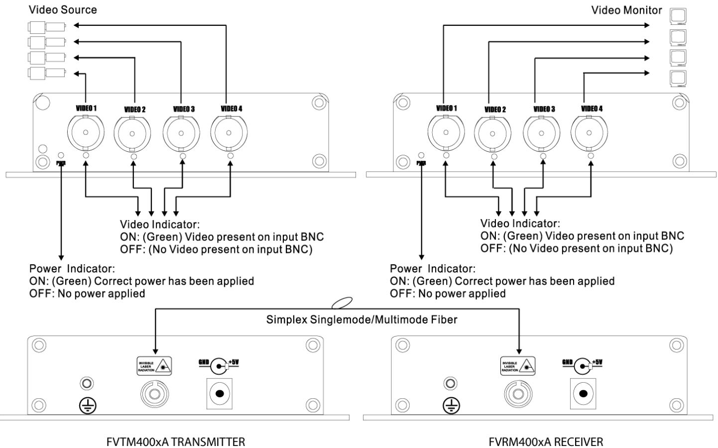
FVTM400xA TRANSMITTER
