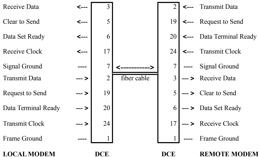
Illustration 7: Modem Link Configuration
