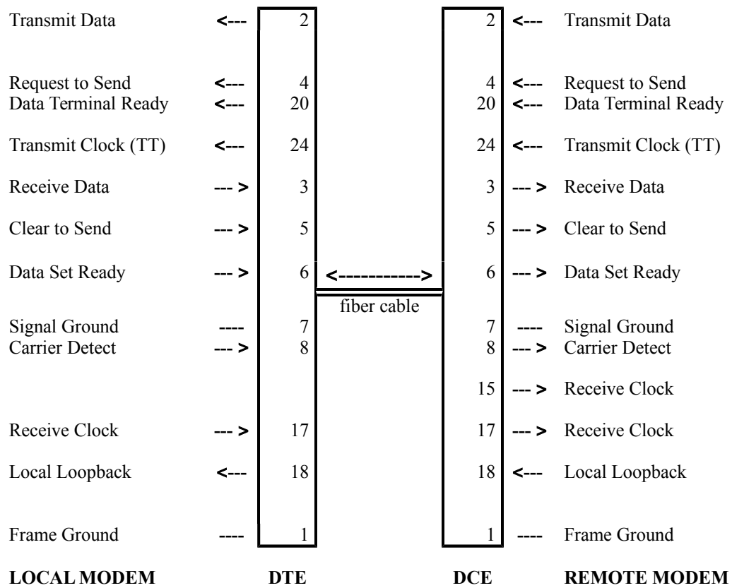
Illustration 5: Interface Extender Configuration(Terminal Timing)
