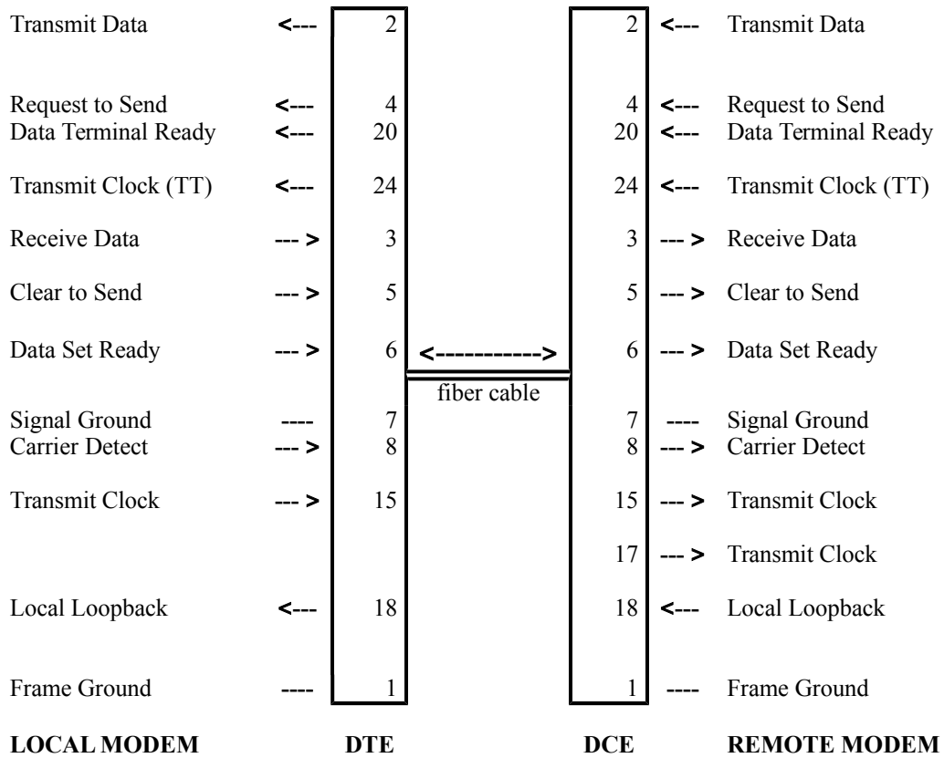
Illustration 6: Interface Extender Configuration(Source Timing; DTE ONLY S1-5 = ON)
