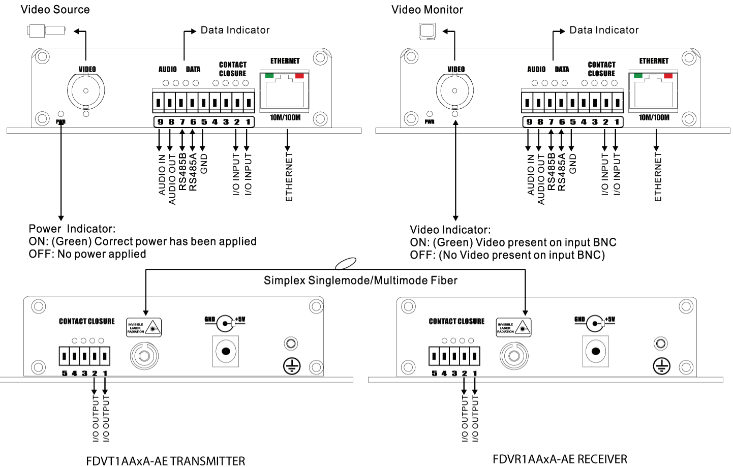
FDVT1AAxA-AE TRANSMITTER
